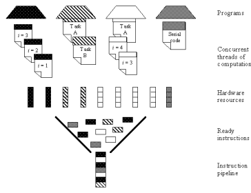
A logical view of a MTA Processor
